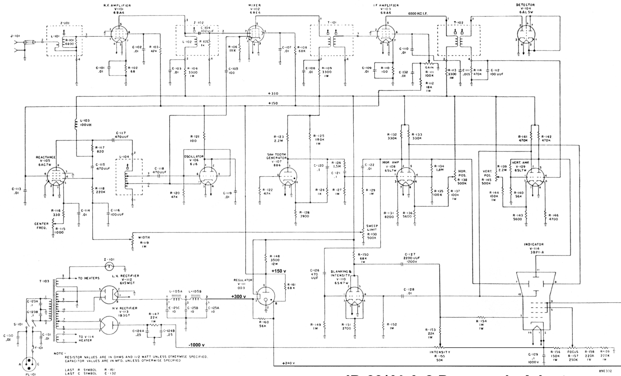
IP-69/ALA-2 Panoramic Adapter
